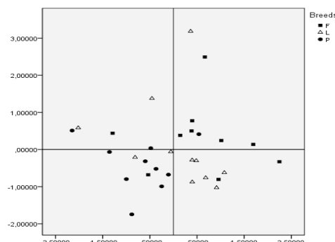
Figure 3. Plot of the first two PC score vectors.
