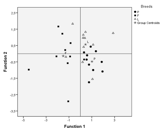
Figure 4. Plot of the two discriminant functions for classification of young bulls according to their breed.
